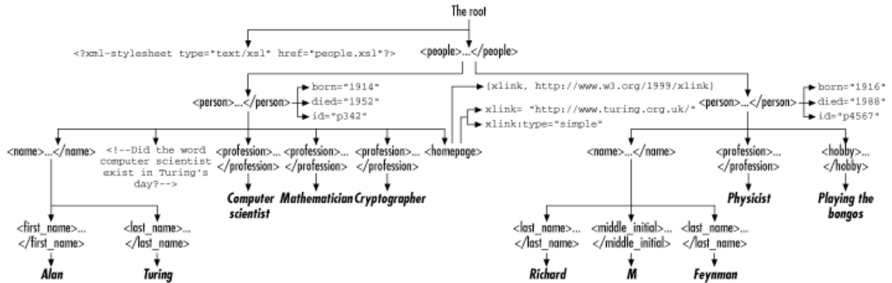
Figure 9-1. The tree structure of Example 9-1
